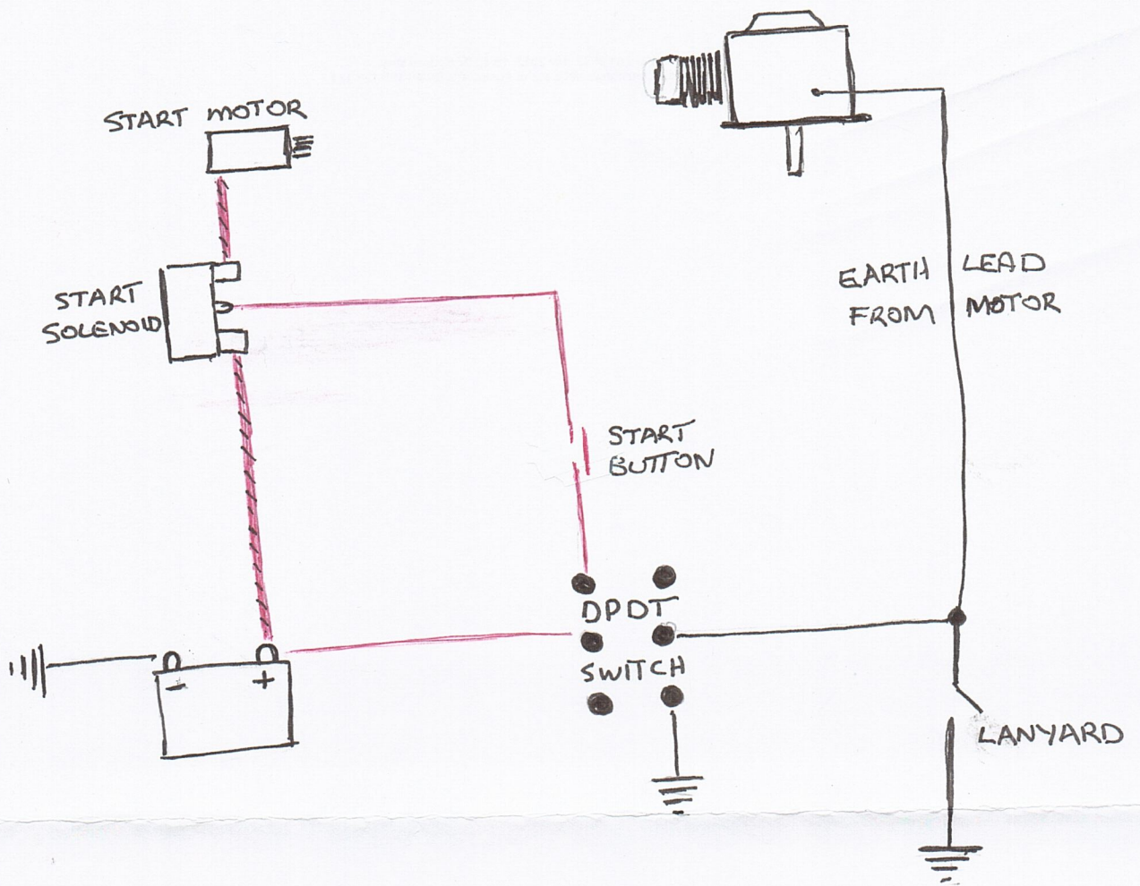
BASIC WIRING FOR BRIGGS & STRATTON IGNITION
